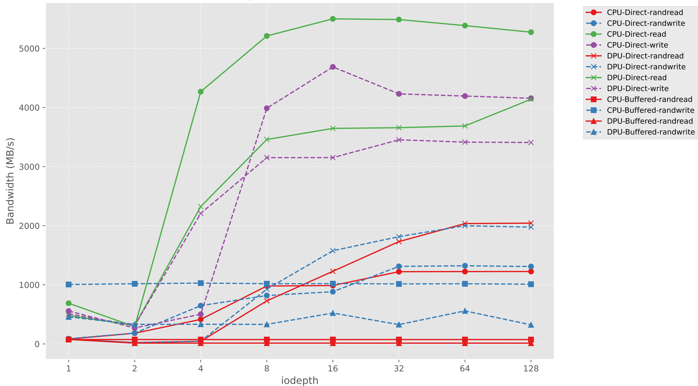
Bandwidth vs iodepth (CPU vs DPU, Direct vs Buffered)
